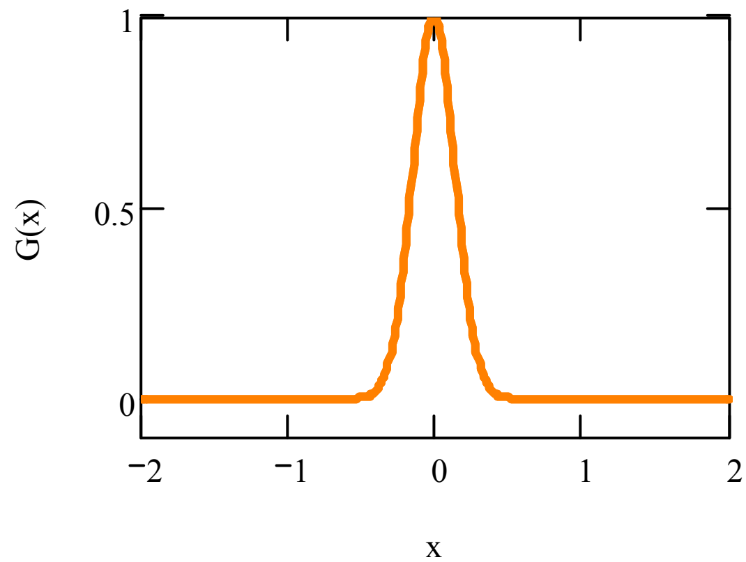
Gaussian Function G_{\sigma}(x)
