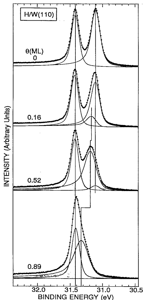
FIG. 2. Three-peak fit of W 4f_{7/2} photoemission spectra for selected H coverages \Theta in monolayers. Intensity of the bulk component at highest binding energy is shown equal for all fits. Bulk and unperturbed-surface line shapes and positions are held constant to their clean-surface values (see Ref. 10), but their amplitudes are allowed to vary with \Theta . Third component (shaded), describing the effect of the H, is unconstrained. Solid circles are the data and the solid line is the fit.
