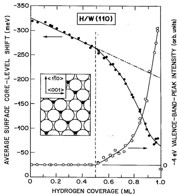
FIG. 3. Average SCS, \bar{E}_s(\Theta) (solid circles), and -4 -eV valence-band (VB) peak intensity (open circles) vs H coverage. Solid lines are drawn as guides to the eye. The dot-dashed line is an extrapolation of the solid line through the data. The dashed vertical line is drawn to contrast the different coverage dependences of the average SCS below and above 0.5 ML. Onset of -4 -eV VB peak indicates 0.5-ML coverage (see Refs. 11 and 15). Inset: W(110) p(2 \times 1) -H surface at 0.5-ML coverage with H at one end of the hourglass site.
