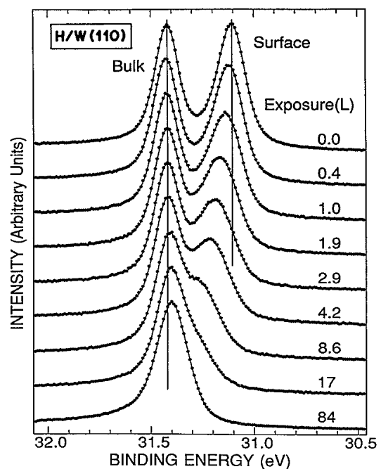
FIG. 1. Photoemission spectra of W 4f_{7/2} electrons for increasing exposures of H in langmuirs (1 L = 10^{-6} Torrsec).
