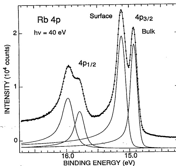
FIG. 2. Analysis of the photoemission spectrum of the 4 p region of Rb metal. The data, taken with the sample at 147 K, are one of a set used to determine the temperature dependence of the phonon width. The components of the bulk and surface spin-orbit doublets are shown separately.
