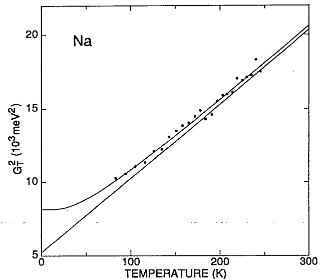
FIG. 4. Fit to the bulk Gaussian width of Na using Eq. (2) (see text).
